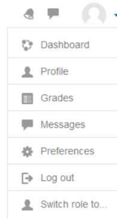
Gambar 4. Setting Moodle
