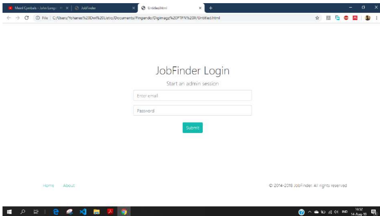
Gambar 4 Login Administrator
