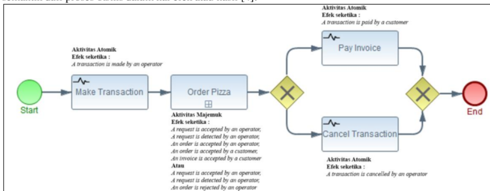
Gambar 2 Model Proses Bisnis Pembelian Pizza
