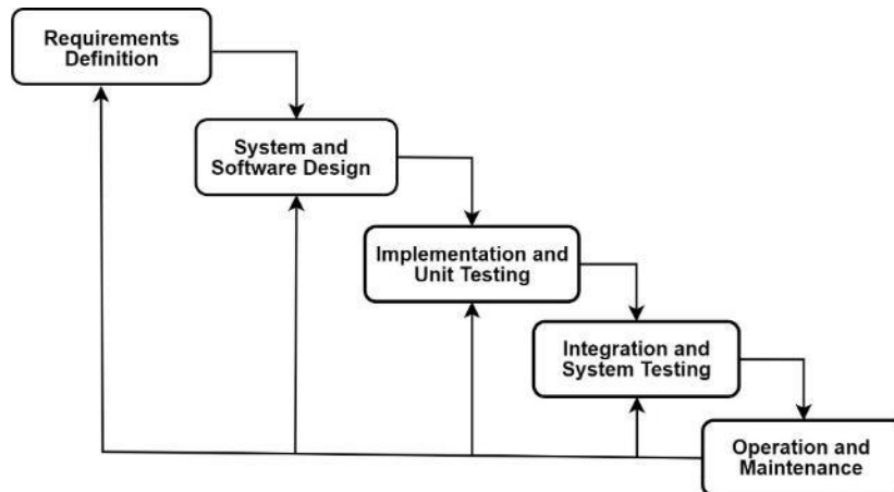
Gambar 1. Prosedur Penelitian
