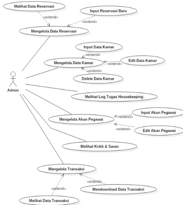
Gambar 3. Usecase Admin
