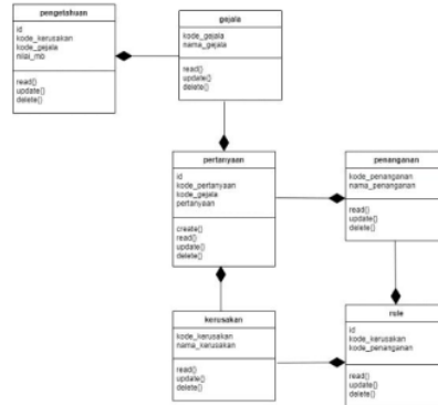
Gambar 8. Class Diagram
