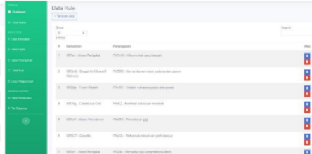
Gambar 14. Halaman Rule
