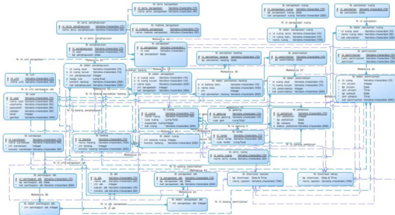
Gambar 2 Conceptual Data Model
