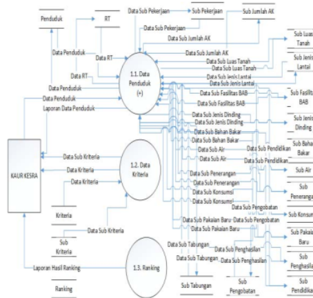
Gambar 4. DFD Level 2 Sub 1
