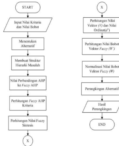
Gambar 1. Flowchart Tahapan Metode FAHP
