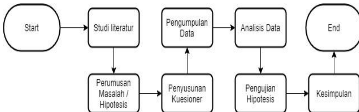
Gambar 1. Alur Penelitian
