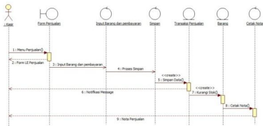
Gambar 7. Sequence Diagram Penjualan
