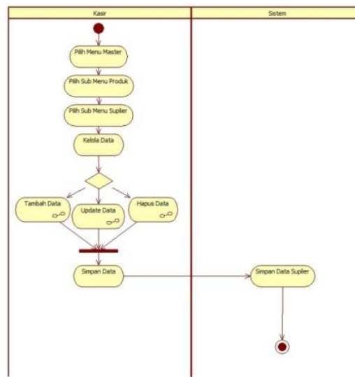
Gambar 5. Activity Diagram Supplier
