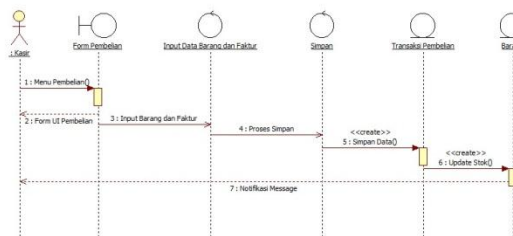
Gambar 8. Sequence Diagram Pembelian
