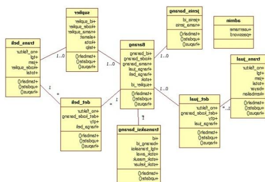
Gambar 9. Class Diagram Sistem
