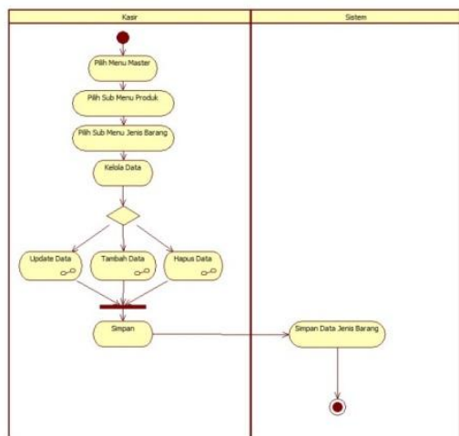
Gambar 4. Activity Diagram Jenis Barang
